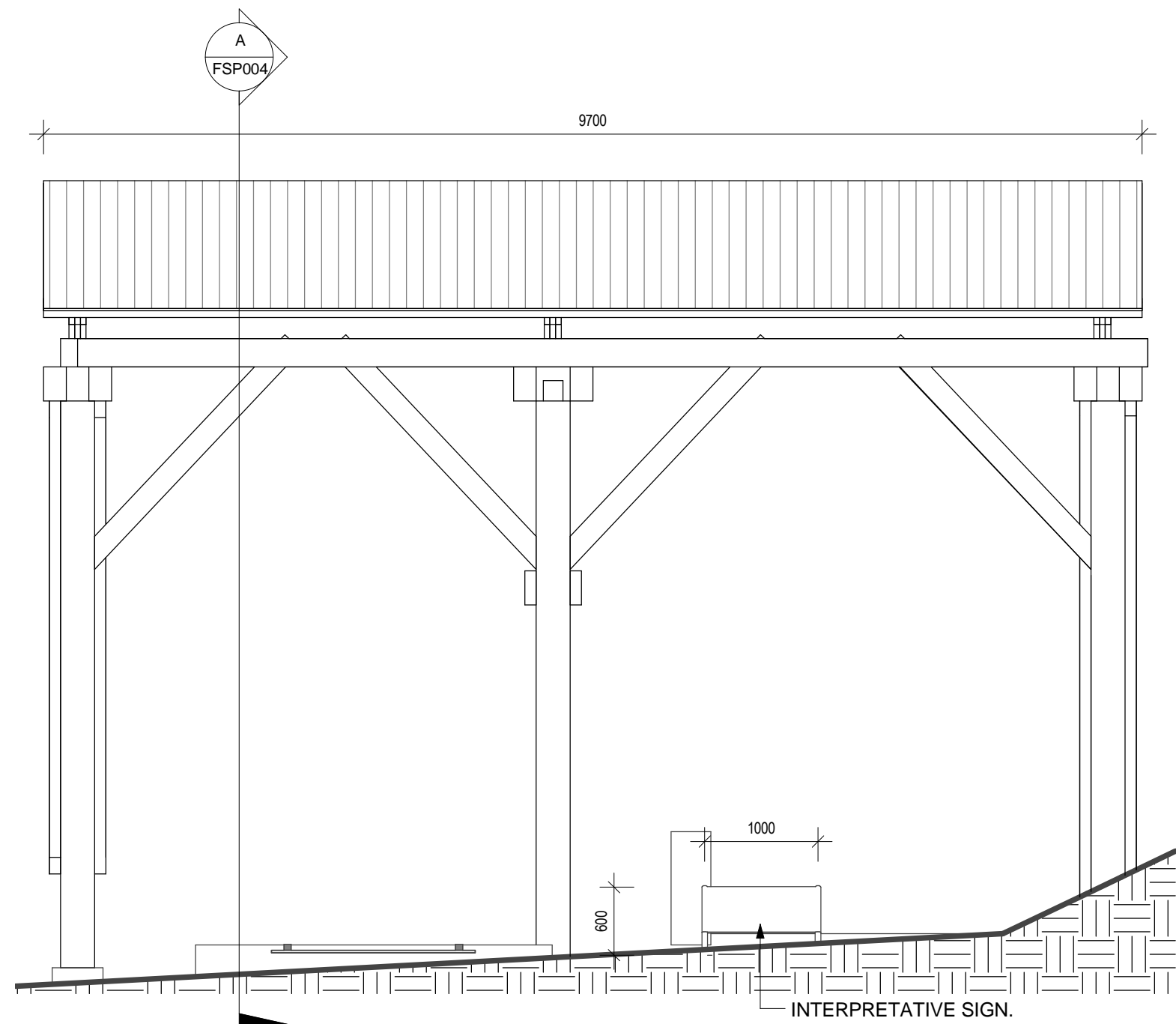
WEIGHBRIDGE NORTH WEST ELEVATION
