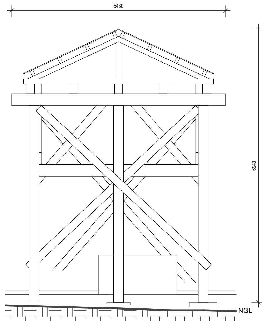
WEIGHBRIDGE NORTH EAST ELEVATION
