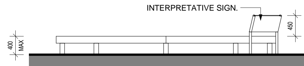
VIEWING PLATFORM SOUTH WEST ELEVATION
